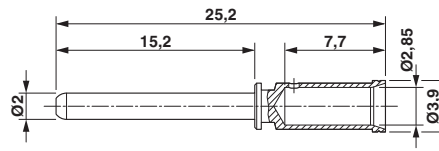
Dimensional drawing
