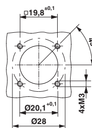
Dimensional drawing
