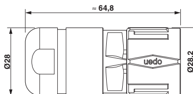
Dimensional drawing
