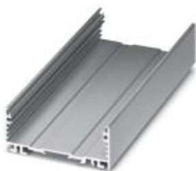
Panel mounting base, Lower part, color: aluminum color, width: 75 mm, length: 235 mm, height: 29.4 mm
