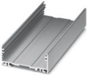
Panel mounting base, Lower part, color: aluminum color, width: 75 mm, length: 990 mm, height: 29.4 mm
