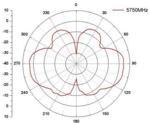
vertical 5750 MHz
