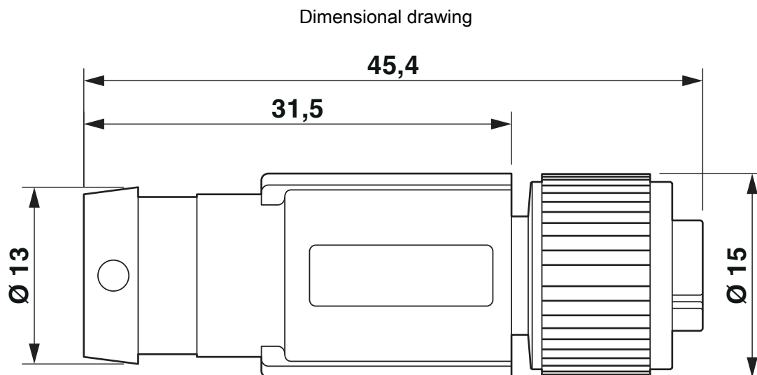
M12 x 1 socket, straight, shielded
